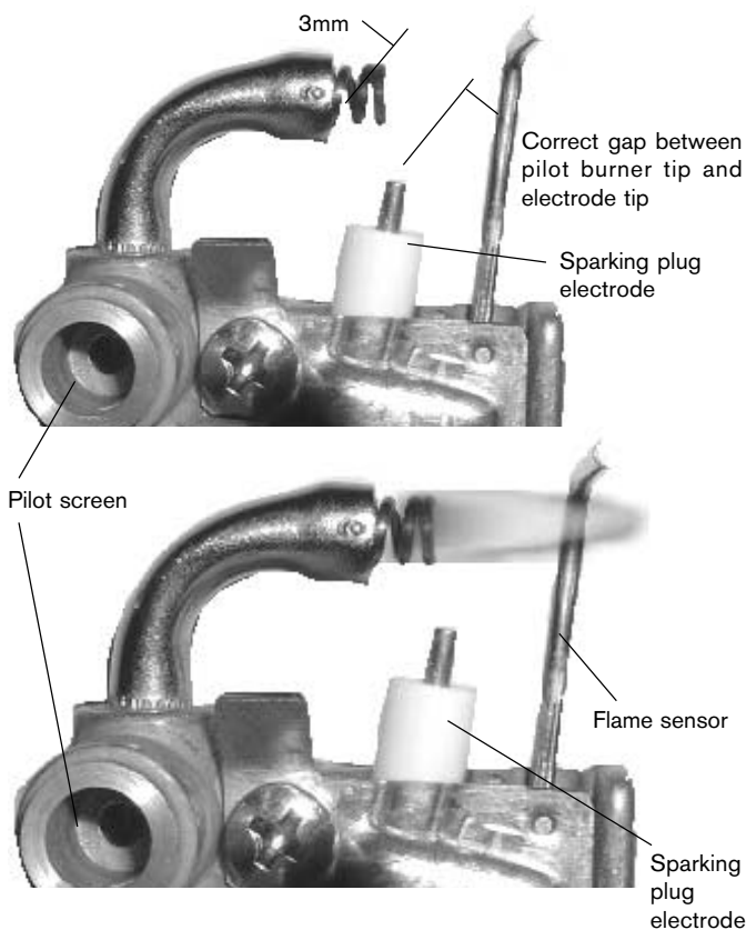
Fig. 12 - Characteristic Pilot Flame
